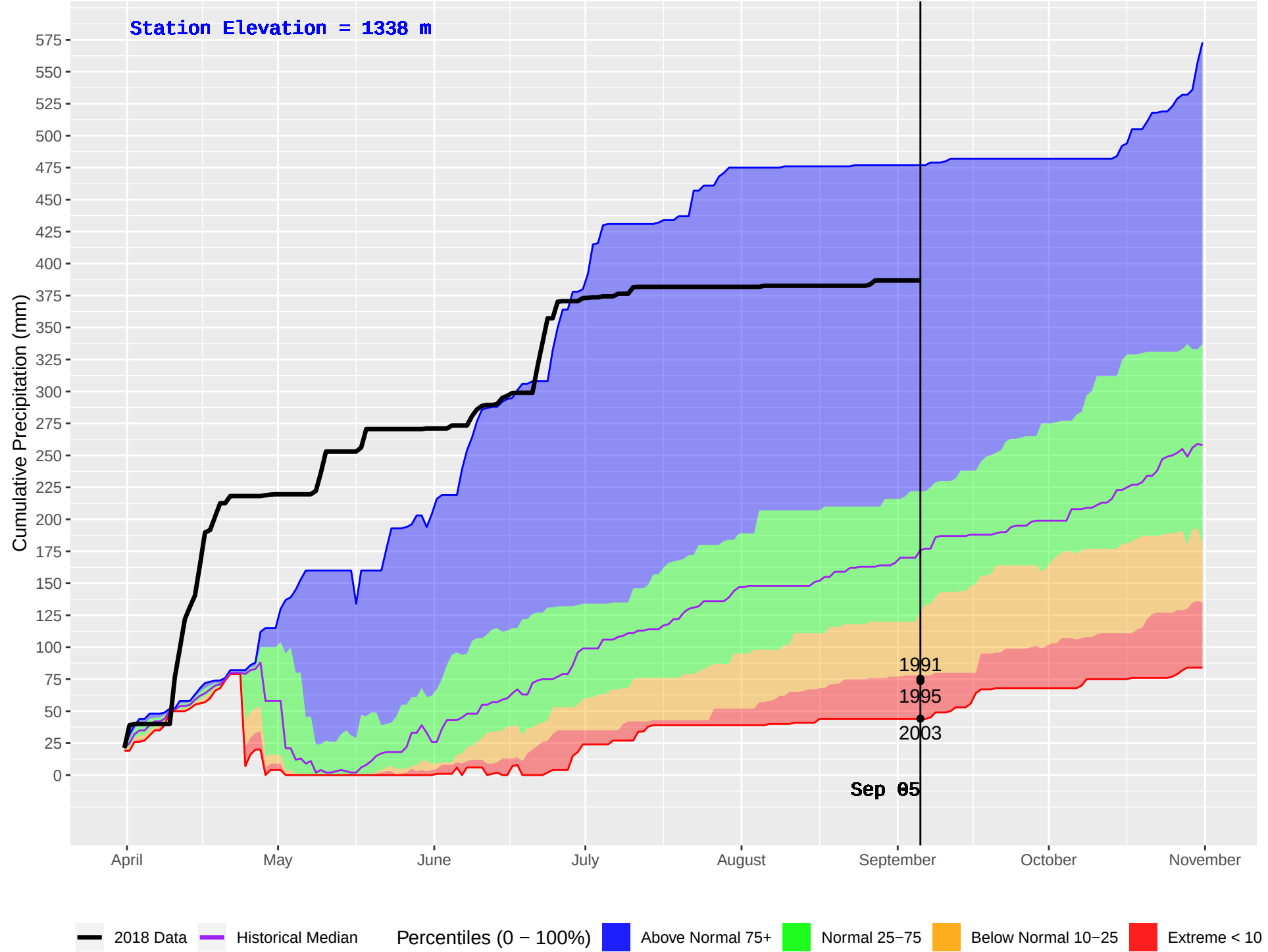
EIGHT MILE (391) : Historical (1980–2016) and Current (2018) Daily Cumulative Precipitation
