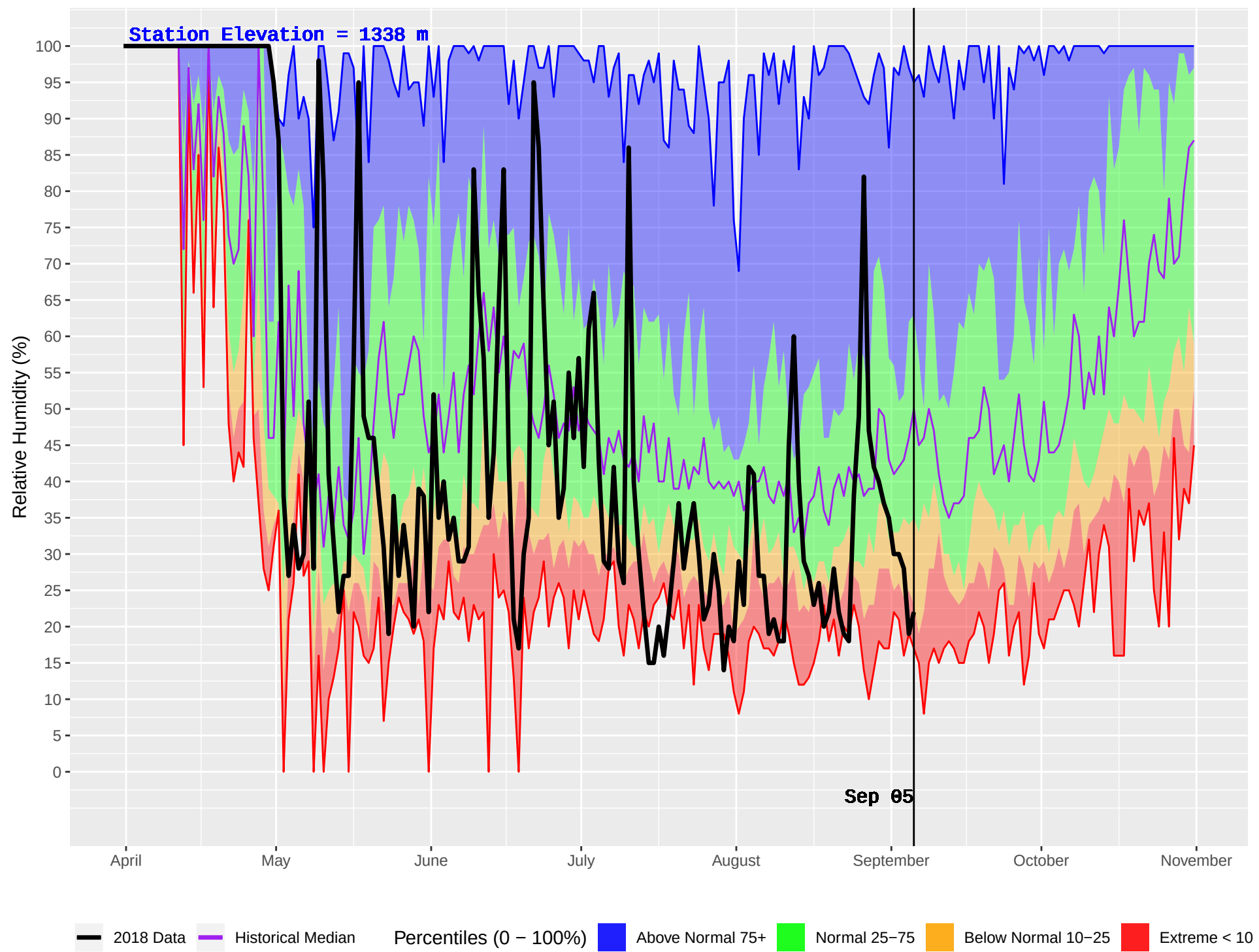
EIGHT MILE (391) : Historical (1980–2016) and Current (2018) Daily Relative Humidity
