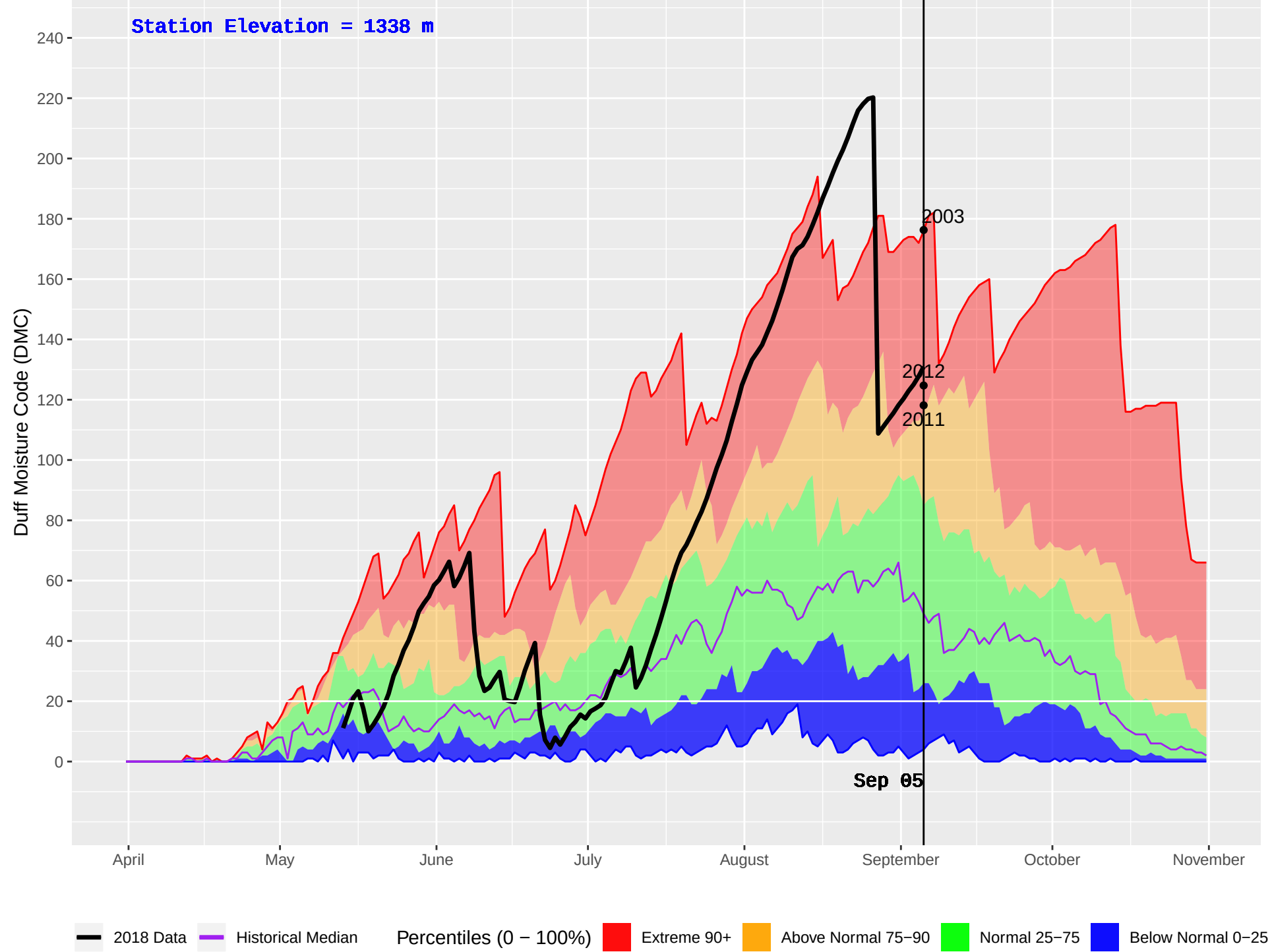
EIGHT MILE (391) : Historical (1980–2016) and Current (2018) Daily Duff Moisture Code (DMC)
