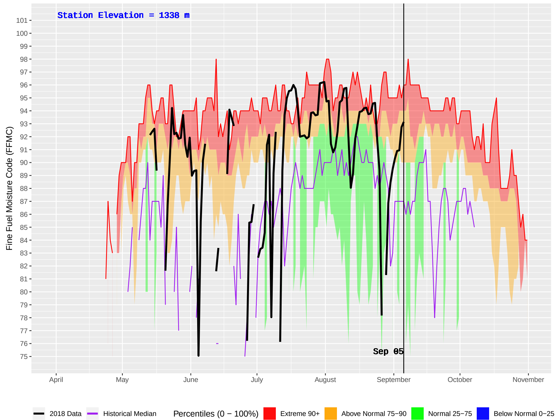
EIGHT MILE (391) : Historical (1980–2016) and Current (2018) Daily Fine Fuel Moisture Code (FFMC)
