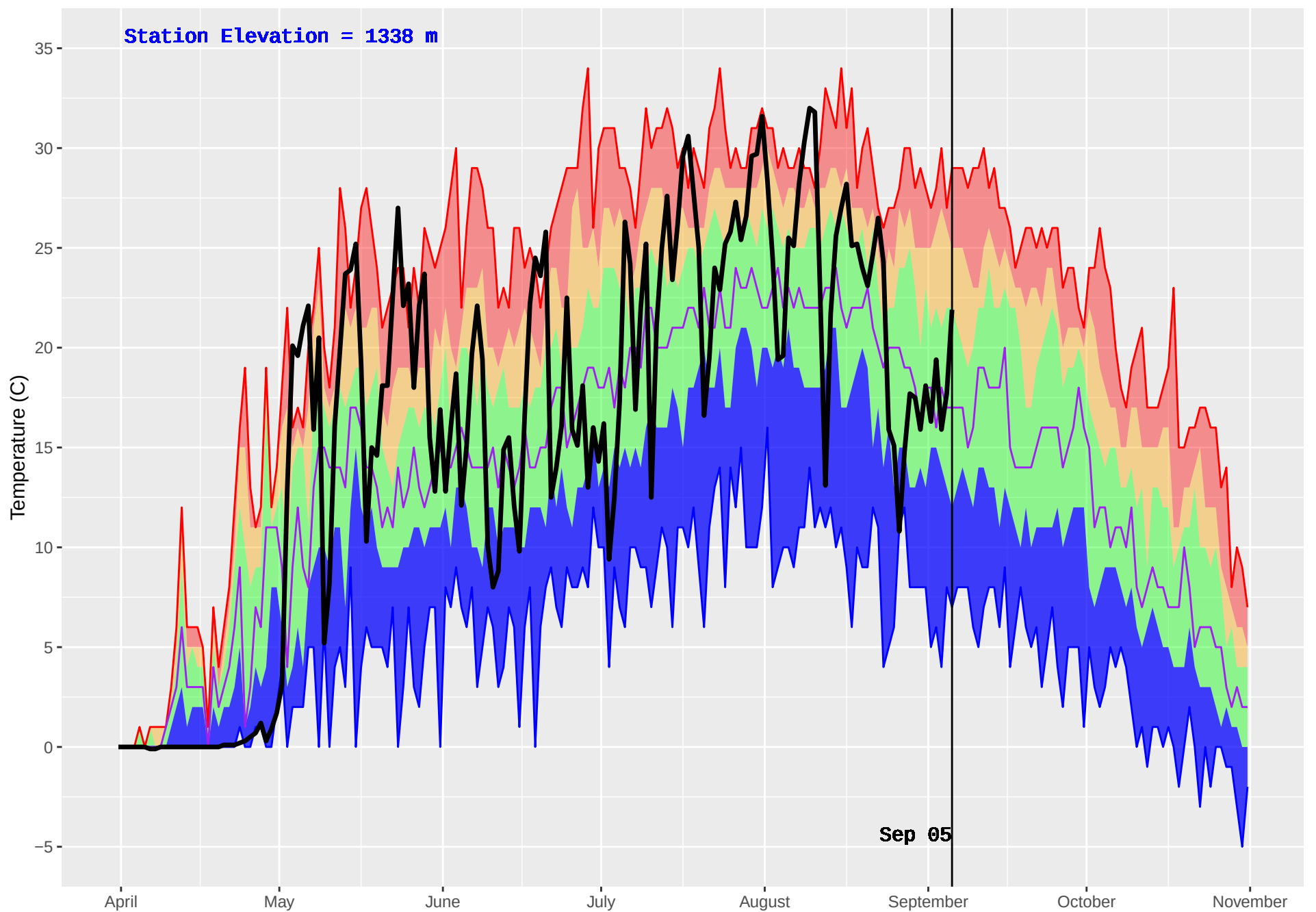
EIGHT MILE (391) : Historical (1980–2016) and Current (2018) Daily Temperature
