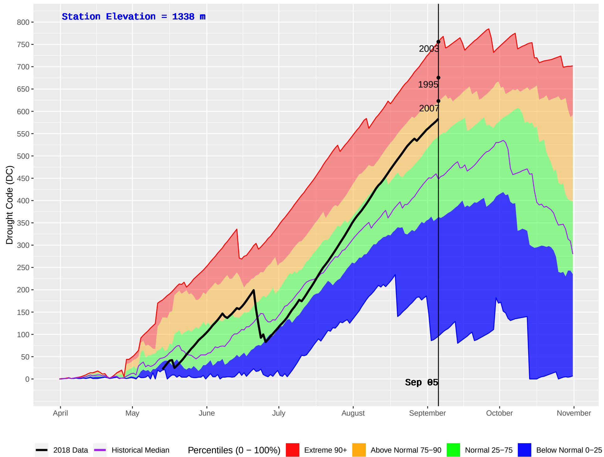
EIGHT MILE (391) : Historical (1980–2016) and Current (2018) Daily Drought Code (DC)
